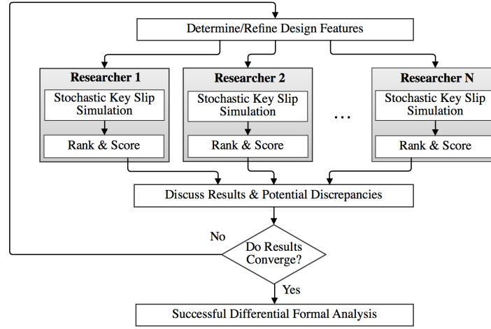
Figure 3: The Differential Formal Analysis Process
