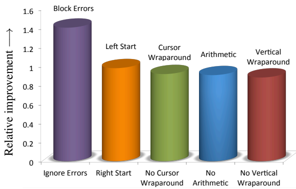
Figure 4: Summary of C# analysis findings. Features mentioned at the top of the bars are better, by the factor shown. Specifically, over all design choices, blocking errors reduces the mean sensitivity of the 5-key interface by a factor of 1.41, start at left is better than start at right by a factor of 0.98, cursor wraparound is better than no cursor wraparound by a factor of 0.91, arithmetic is better than no arithmetic by a factor of 0.9 and vertical wraparound gives us an improvement over no vertical wraparound by a factor of 0.88.
