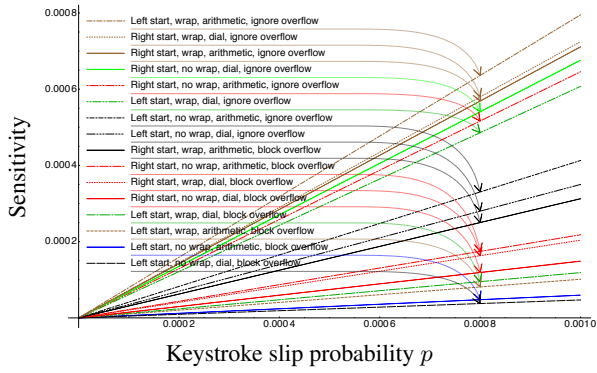
Figure 5: Sensitivity against p for various combinations of design feature (from Mathematica ). The lower gradient lines represent better (less error-sensitive) designs.
