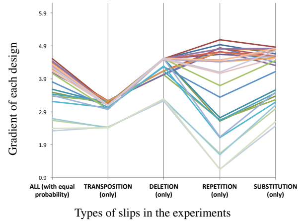
Figure 6: Parallel Coordinates visualisation showing the relation of design rankings depending on slips
