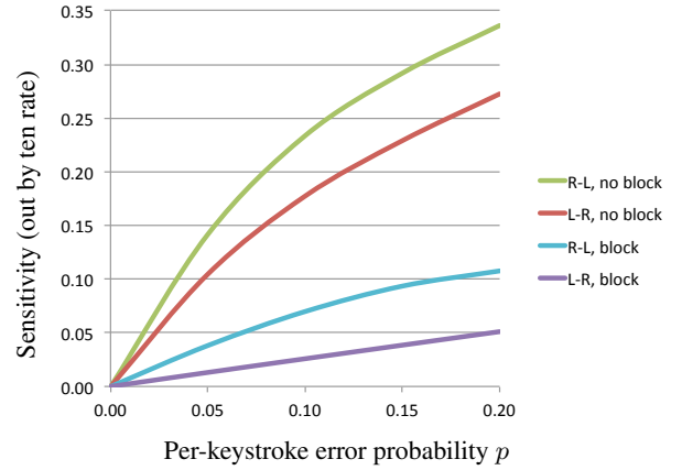
Figure 8: Results for BBraun experiments: entry left-to-right admits less out-by-10 errors than right-to-left, and blocking errors reduces out-by-10 errors still further.
