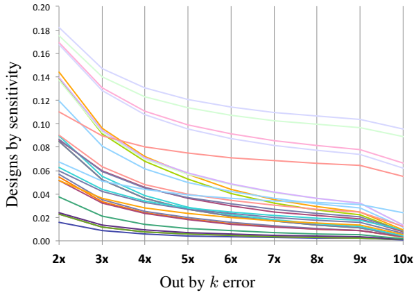
Figure 7: Out by k errors for different design types.
