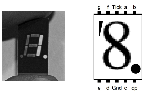
Figure 16. Envisioning how the legibility of a typical standard seven segment package (left) could be improved with a pin-compatible high resolution display (right; the pin letters a–g are the standard segment identifiers). Using BCD (instead of one pin per segment) or a pre-defined seven segment font would allow unambiguous display of hexadecimal digits. An extra pin could also be used to select a smaller font for fractional digits.
